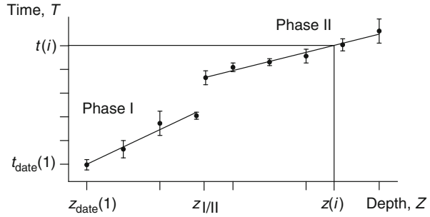
Fig. 4.4 Two-phase linear timescale model. The break in the accumulation occurs at depth z_{I/II} . See also Fig. 4.3
