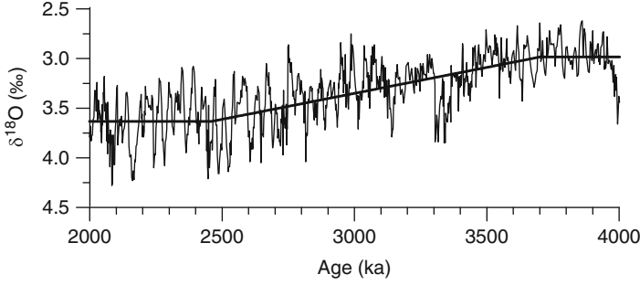
Fig. 4.6 Ramp regression of the marine \delta^{18}\text{O} record ODP 846 (Fig. 1.3). The long-term trend (thick line) documents the Northern Hemisphere Glaciation. The estimated change-points ( \pm standard errors) of this climate transition are \hat{t}_1 = 2462 \pm 129 ka, \hat{x}_1 = 3.63 \pm 0.04 ‰, \hat{t}_2 = 3700 \pm 119 ka and \hat{x}_2 = 2.99 \pm 0.04 ‰. The estimates were obtained by WLS using iteratively updated variability. Also S(i) was given a ramp form ( \hat{S}(i) = 0.27 ‰ for t(i) \leq 2600 ka, 0.18 ‰ for t(i) > 3550 ka and linearly connected between these change-points). The standard errors given here are from SB resampling (Sect. 3.8) using B = 400 and an average block length equal to \hat{\tau} = 7.7 ka. A rough method to take into account the timescale uncertainty of 25 ka is Gaussian error propagation (Mudelsee and Raymo 2005), yielding total errors of (129^2 + 25^2)^{1/2} ka \approx 131 ka (for \hat{t}_1 ) and (119^2 + 25^2)^{1/2} ka \approx 122 ka (for \hat{t}_2 ) (After Mudelsee and Raymo 2005)
