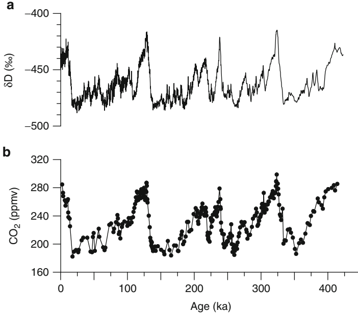
Fig. 1.4 Ice core data: deuterium and CO 2 records from the Vostok station (Antarctica) over the past 420,000 years. The core was drilled into the ice (diameter, 12 cm; length, 3623 m) and recovered in segments. The deuterium record (a) was measured on ice material using a mass spectrometer. Values are given in delta notation: \delta D = [(D/H)_{\text{sample}} / (D/H)_{\text{SMOW}} - 1] \cdot 1000 \text{ ‰} , where (D/H) is the number of D particles over the number of H particles and SMOW is “Standard Mean Ocean Water” standard. Total number of points, n , is 3311. The CO 2 record (b) was measured on air bubbles enclosed in the ice. Values are given as “parts per million by volume”, n is 283. In (b), values (dots) are connected by lines; in (a), only lines are shown. The present-day CO 2 concentration ( \sim 389 ppmv in the year 2010) is not recorded in (b). The construction of the timescale (named GT4) was achieved using a model of the ice accumulation and flow. Besides glaciological constraints, it further assumed that the points at 110 and 390 ka correspond to dated stages in the marine isotope record. Construction of the CO 2 timescale required additional modelling because in the ice core, air bubbles are younger in age than ice at the same depth. One climatological question associated with the data is whether variations in CO 2 (the values in air bubbles presenting the atmospheric value accurately) lead over or lag behind those of deuterium (which indicate temperature variations, low \delta D meaning low temperature) (Data from Petit et al. 1999)
