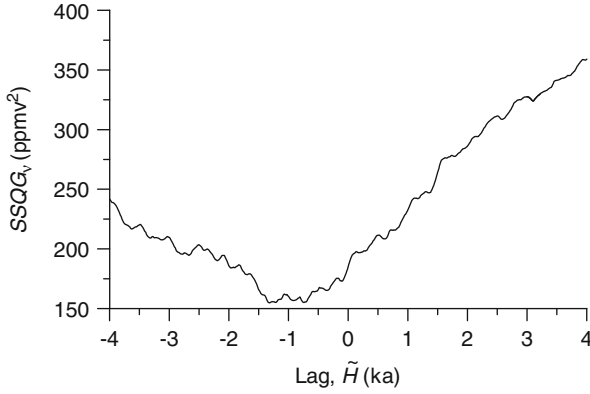
Fig. 8.11 Vostok deuterium and CO 2 , reduced sum of squares. The minimum (i.e. lag estimate) is at \tilde{H} = -1.3 ka (After Mudelsee 2001b)
