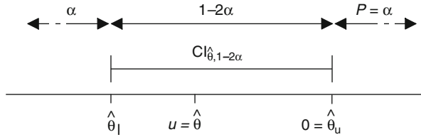
Fig. 3.5 Hypothesis test and confidence interval. The parametric null hypothesis H_0 : “ \theta < 0 ” cannot be rejected against H_1 : “ \theta \geq 0 ” with a P -value equal to \alpha
