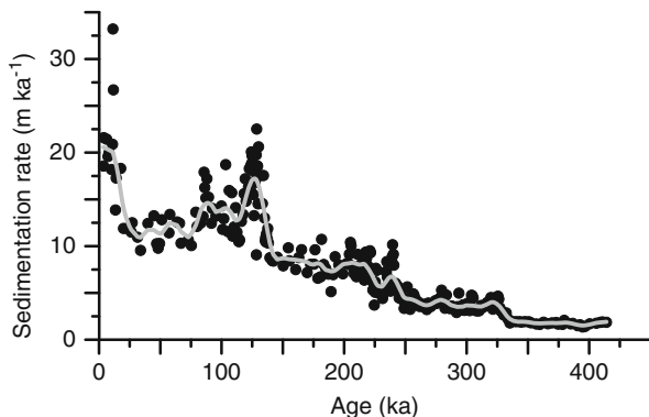
Fig. 4.13 Nonparametric regression of the sedimentation rate in the Vostok record. The sedimentation rate ( dots ) \dot{z} = [z(i+1) - z(i)]/[t(i+1) - t(i)] , where z is depth, is calculated from the \text{CO}_2 data on the GT4 timescale (Fig. 1.4b). (Strictly speaking, \dot{z} refers not to the “sedimentation” of the ice but to the derivative of the depth–age curve after ice accumulation and compaction.) The smoothed curve ( solid grey line ) is \hat{x}_{\text{trend}}^{\text{GM}}(t) calculated with a parabolic kernel, a cross-validated bandwidth of h = 8 ka and boundary adjustments (“boundary kernel”)
