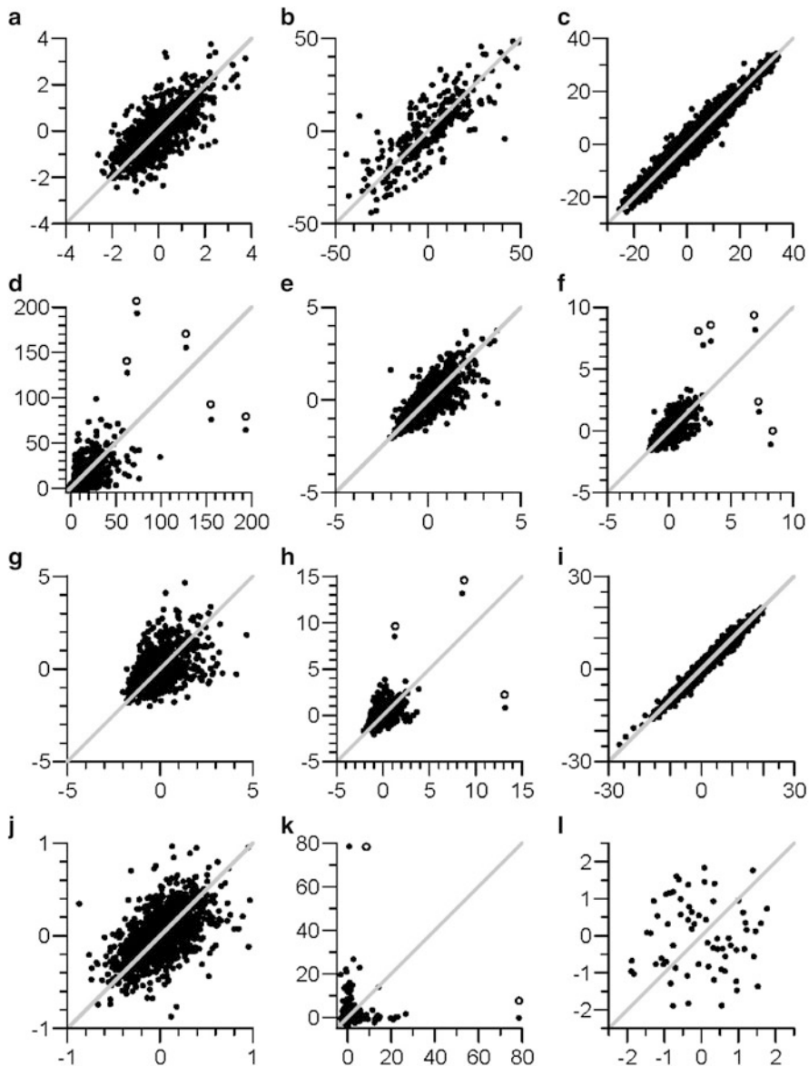
Fig. 1.13 Persistence of noise in selected climate time series. (a) ODP 846 \delta^{18}\text{O} ; (b) Vostok \text{CO}_2 ; (c) Vostok \delta\text{D} ; (d) NGRIP \text{SO}_4 ; (e) NGRIP \text{Ca} ; (f) NGRIP dust content; (g) NGRIP electrical conductivity; (h) NGRIP \text{Na} ; (i) tree-ring \Delta^{14}\text{C} ; (j) Q5 \delta^{18}\text{O} ; (k) Lower Mystic Lake varve thickness; (l) HadCM3 runoff. Noise data are shown as lag-1 scatterplots (in each panel, x(i-1) is plotted on the ordinate against x(i) on the abscissa as points ), together with 1:1 lines (grey). Data and units are given in Figs. 1.3–1.10. Detrending and S(T) normalization prior to analysis were carried out as in Fig. 1.12. Note that in (d), all points are shown (unlike as in Fig. 1.12d). Outliers are tentatively marked with open circles
