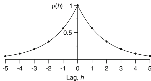
Fig. 2.2 Autocorrelation function of the AR(1) process, a > 0 . In the case of even spacing (Sect. 2.1.1), \rho(h) is given by a^{|h|} = \exp[-|h| \cdot d/\tau] , and in the case of uneven spacing (Sect. 2.1.2), by \exp[-|T(i+h) - T(i)|/\tau] . In both cases, the decrease is exponential with decay constant \tau
