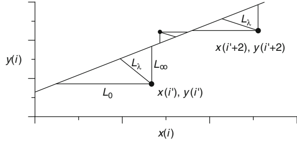
Fig. 8.3 Geometric interpretation of WLSXY.
