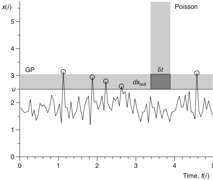
Fig. 6.11 Estimation area for extreme value time series. The area (dark shading) is given by dx_{\text{out}} \cdot \delta t . In the GP case, where POT values (circles) are analysed, \delta t = [t(n) - t(1)] ; in the inhomogeneous Poisson case, where event times are analysed, dx_{\text{out}} \rightarrow \infty . u , threshold; x_{\text{out}}(i) = x(i) - u
