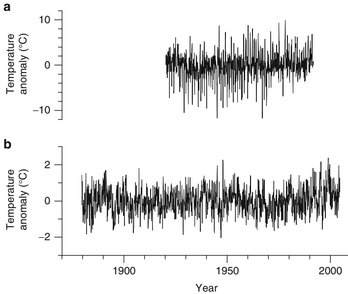
Fig. 1.11 Measured data: surface air temperature records from Siberia (a) and North Atlantic (b). Data are monthly temperature anomalies with respect to the 1961–1990 means from a gridded, global set. Siberia is presented by the grid cell 50–55°N, 90–95°E, effectively reflecting station Krasnoyarsk; the North Atlantic by 35–40°N, 25–30°W. Shown are the gap-free time intervals (a May 1920 to November 1991, n = 859 ; b July 1879 to July 2004, n = 1501 ). The annual cycles were removed by subtracting the monthly averages (Raw data from Jones and Moberg 2003)
