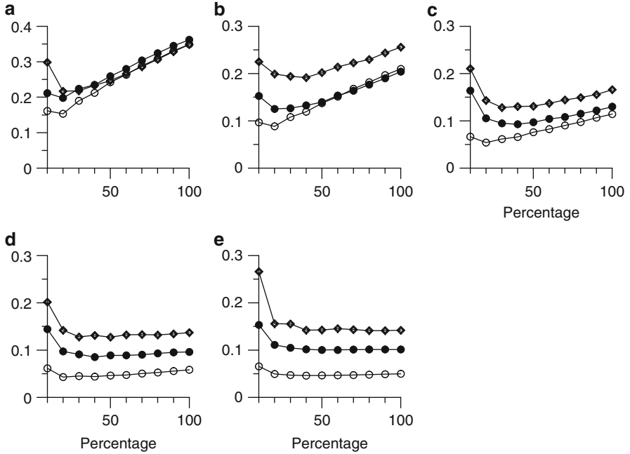
Fig. 7.7 Monte Carlo study of synchrony Pearson's correlation coefficient for unequal timescales, dependence on percentage. (a) \tau_X = \tau_Y = 5 ; (b) \tau_X = \tau_Y = 10 ; (c) \tau_X = \tau_Y = 20 ; (d) \tau_X = \tau_Y = 50 ; (e) \tau_X = \tau_Y = 100 ; (a–e) wildly mixed unequal timescales and \rho_{XY} = 0.8 . See Fig. 7.4 as regards timescale and time series generation. Each panel shows for n = 100 (open diamonds), 200 (filled circles) and 1000 (open circles) the empirical \text{RMSE}_{\tilde{r}_{XY\beta 100\%}} in dependence on the percentage (i.e. \beta )
