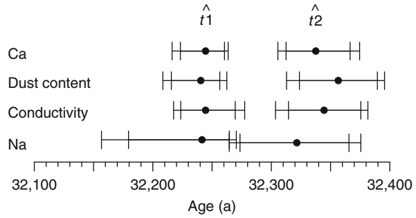
Fig. 4.8 Onset of Dansgaard–Oeschger event 5, NGRIP ice core: estimated change-points with confidence intervals. Shown are 95 and 90 % BCa CIs for \hat{t}_1 and \hat{t}_2 , calculated with ARB resampling
